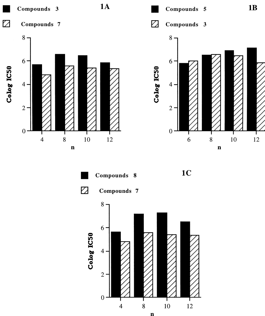
Figure 1. Influence of different parameters on the AChE inhibition as \text{Colog IC}_{50} (i.e. -\log \text{IC}_{50} ) versus chain length ( n ). (A) Linkage effect: N -phthalimido compounds 3 versus O -phthalimido compounds 7 . (B) Terminal group effect: N -alkylammonium derivatives 5 versus N -phthalimido derivatives 3 . (C) Iminium function effect: charged O -phthalimido compounds 8 versus neutral parent compounds 7 .
