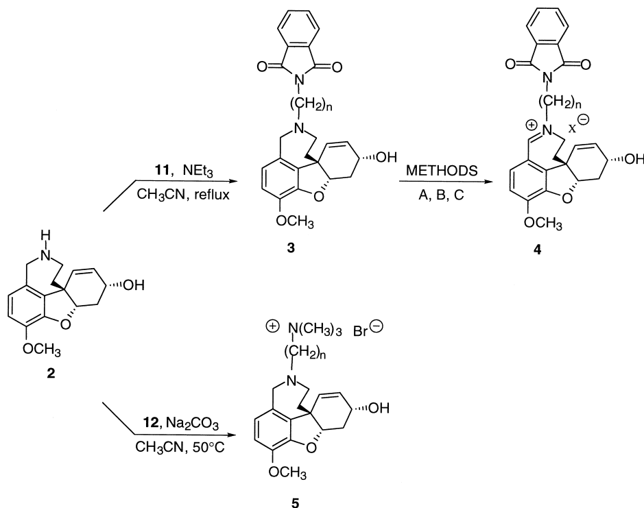
Scheme 3. Method A for 4b–c : (i) m -CPBA 1.1 equiv, CH 2 Cl 2 , 20 °C, 1.5 h; (ii) (CF 3 CO) 2 O, CH 2 Cl 2 , 0 °C, 6 h. Method B for 4d–e : NBS-AIBN, CCl 4 , 20 °C. Method C for 4f : (i) I 2 , NaOAc, EtOH, reflux, 1 h; (ii) HBr, 0.5% solution in water.
